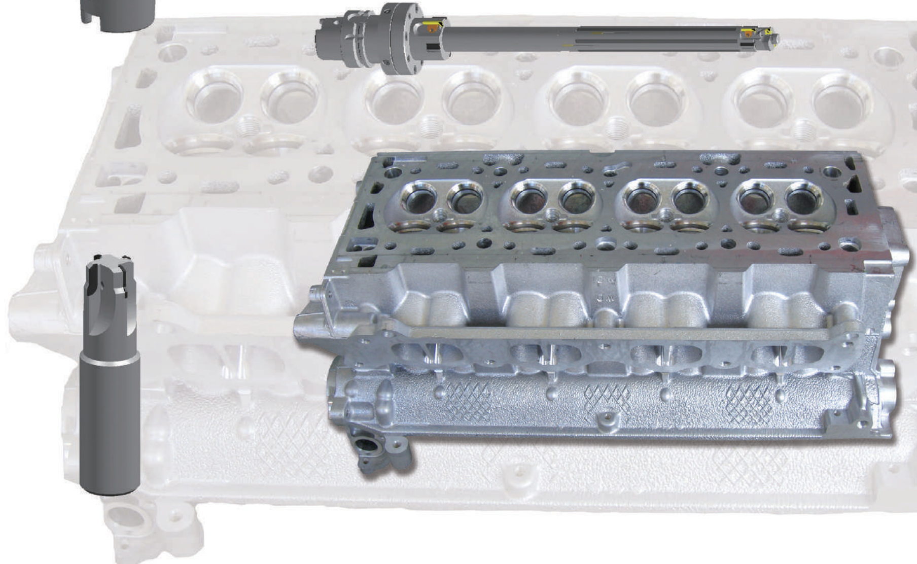
• CAMSHAFT BEARING FINISH BORING TOOL
